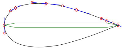
FIGURE 4.2. Parameterised obstacle shape (NACA0040)
