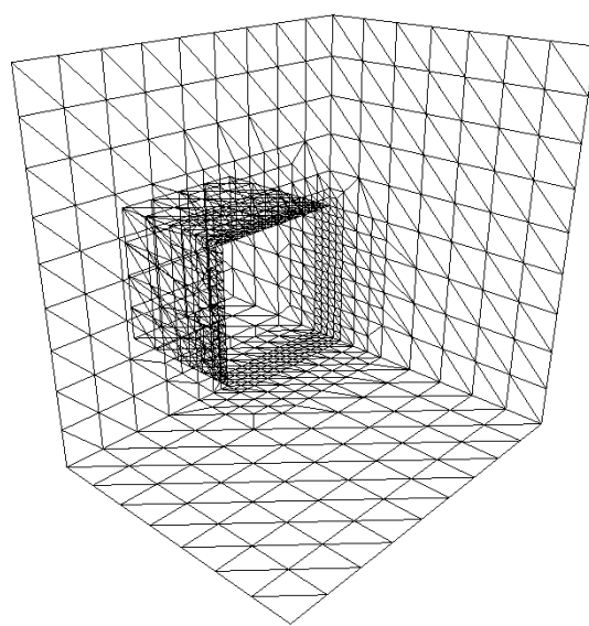
Figure 8: Coarse mesh refined to capture initial shock.
