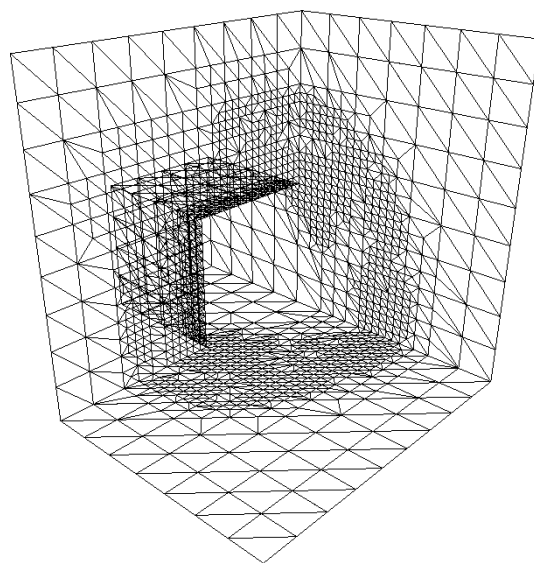
Figure 9: Adapted mesh after 240 time-steps.
